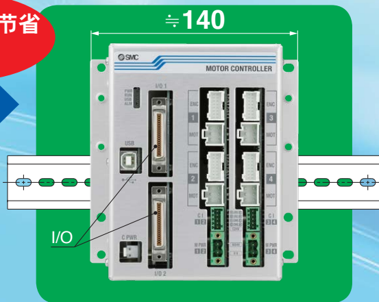
JXC73/83
